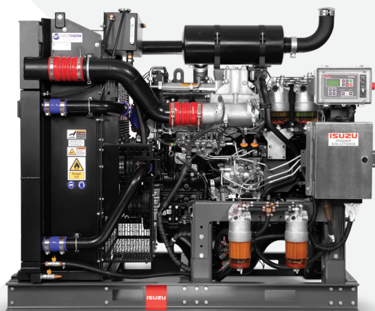
COMMON RAIL ENGINE
